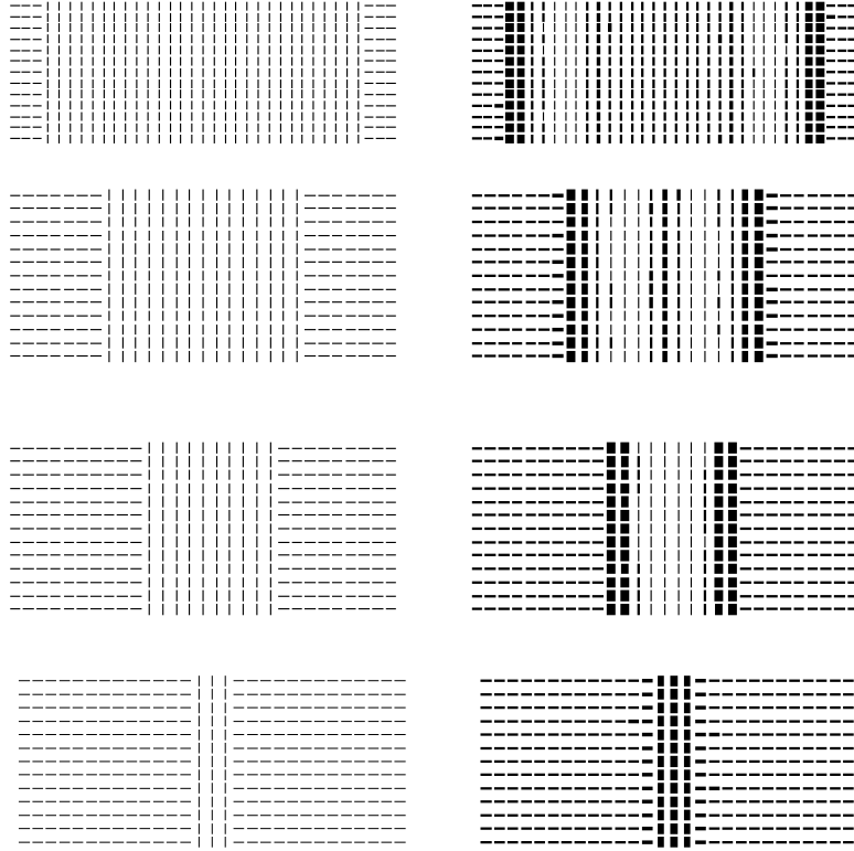
Figure 3: Dependence on the size of the figure. The figure-ground effect is most evident only for small figures, and the medial axis effect is most evident only for figures of finite and appropriate sizes.
